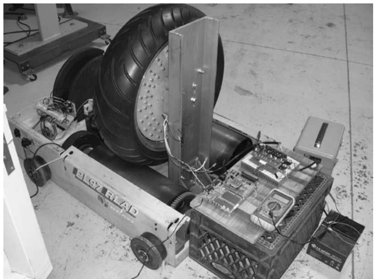
Wheel motor on a dynamometer
