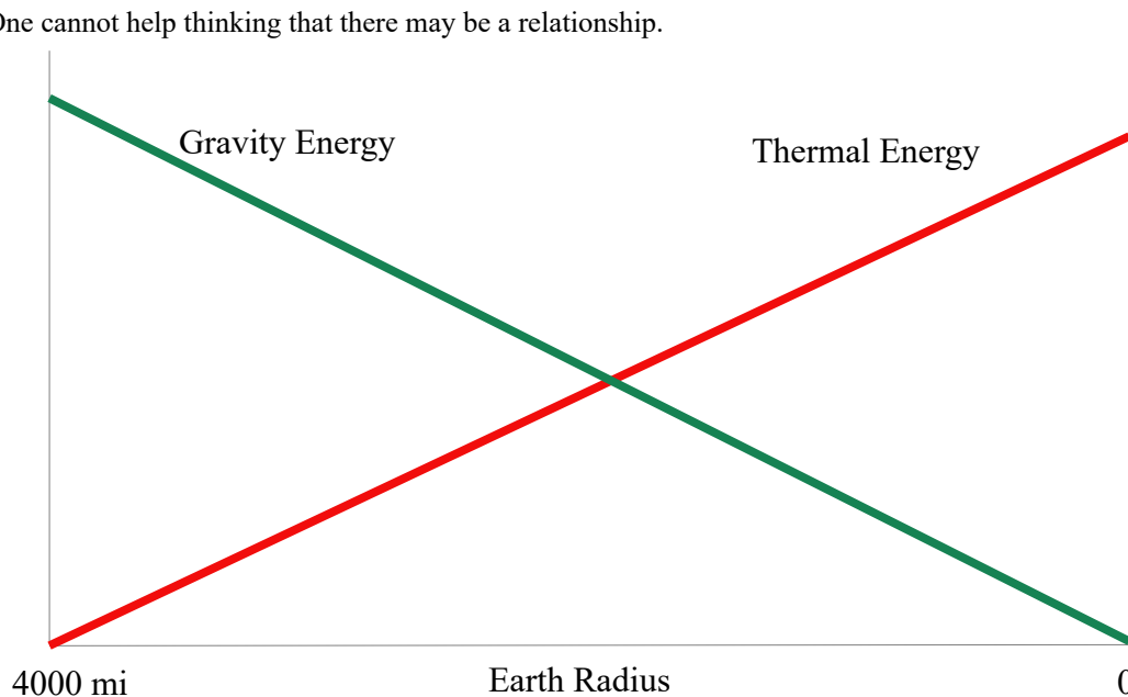
Figure 2. Gravity energy and thermal energy versus Earth Radius.
